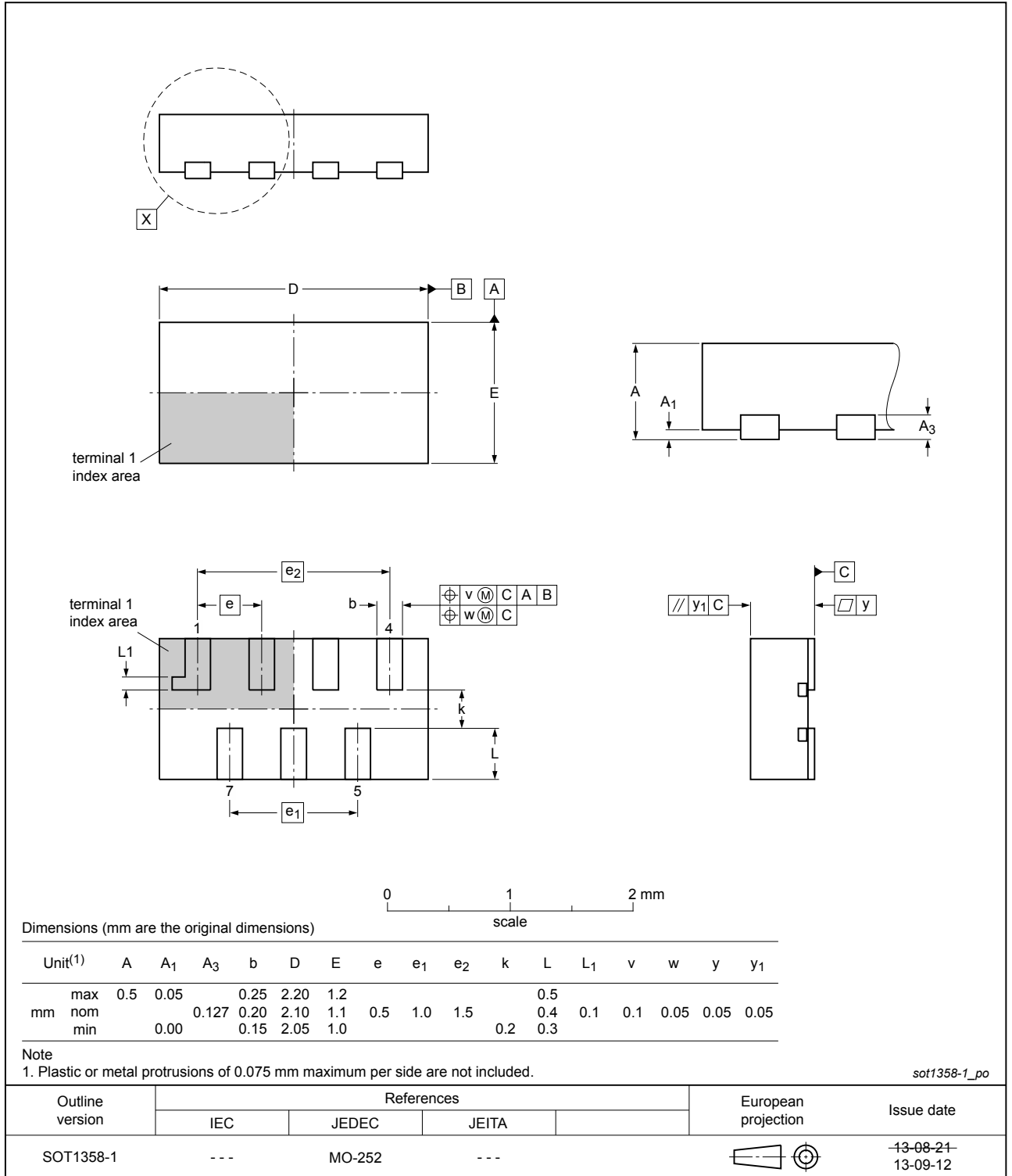
Fig. 1. Package outline XSON7 (SOT1358-1)
